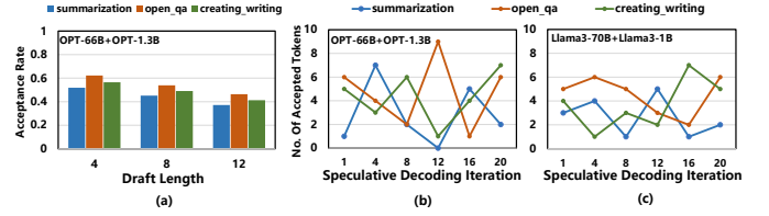
Fig. 4. (a) Token acceptance rates of the OPT-66B + OPT-1.3B model pair across three task categories in the Dolly dataset under different fixed draft lengths. (b) Per-iteration distribution of accepted tokens during speculative decoding for each task category using OPT-66B + OPT-1.3B. (c) Same as (b) using LLaMA3-70B + LLaMA3-1B. The results reveal dynamic and task-specific variations in optimal draft lengths across iterations and model pairs.
