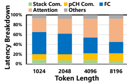
Fig. 17. The execution time breakdown of SADDLE's TLM verification phase
